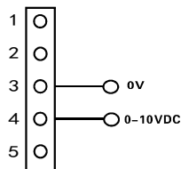
②.0-10V
